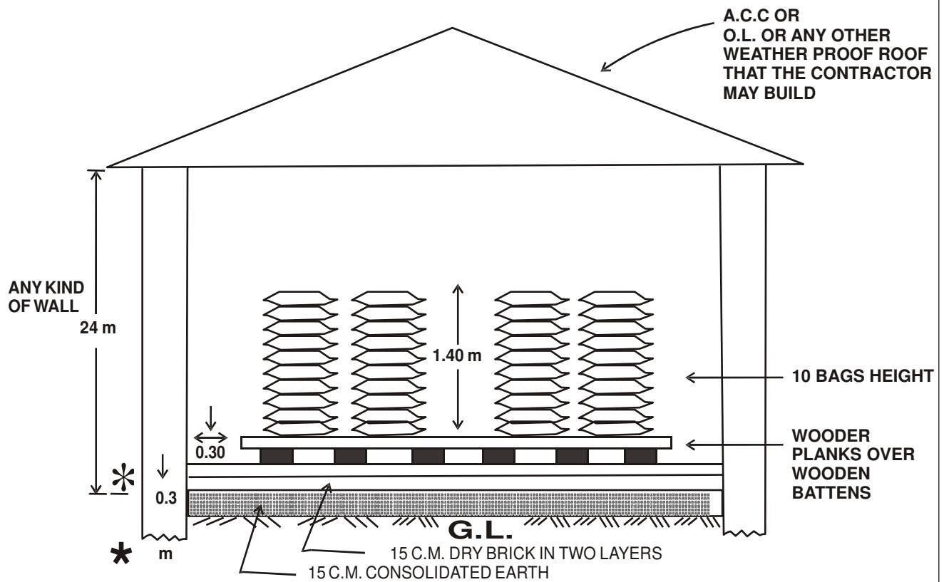
SECTION AB
